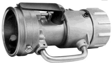
100mm Coupling BSP Female Inlet
